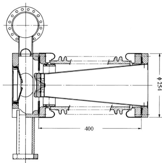
Fig. 11. Electron gun.
