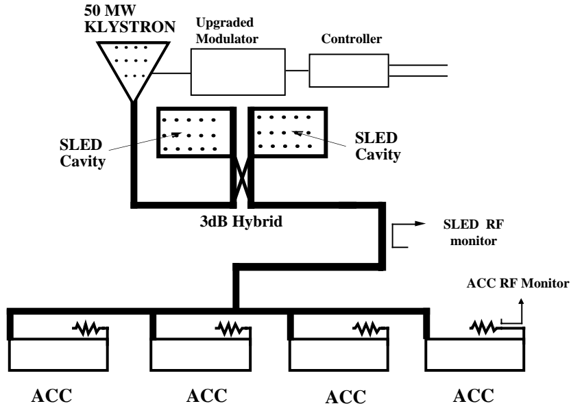
Fig. 9. Schematic diagram of the rf pulse compressor.
